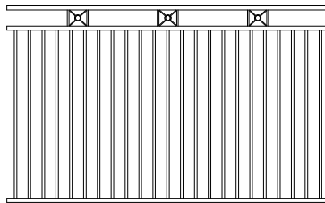
GEMINI (max 3/panel)- 38x25 Rail - 16mm round pickets
