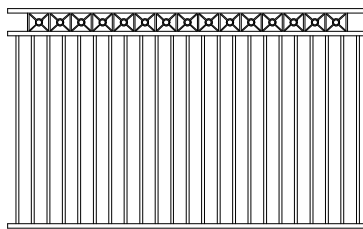
SOUTHERN CROSS - 38x25 Rail - 16mm round pickets
