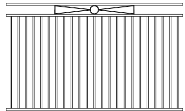
SPLAY (1 per panel) - 38x25 Rail - 16mm round pickets
