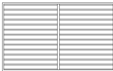
70/19 Horizontal Slat - 70mm blade with 19mm space
