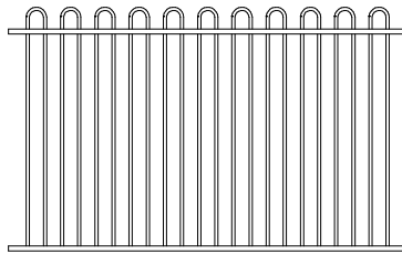
LOOP TOP - 38x25 Rail - 16mm round pickets
