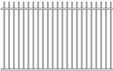
ROD TOP- 38x25 Rail - 16mm round pickets
