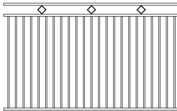
DIAMOND (max 3/panel)- 38x25 Rail- 16mm round pickets
