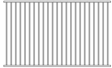
FLAT TOP - 38x25 Rail with 16mm round pickets
